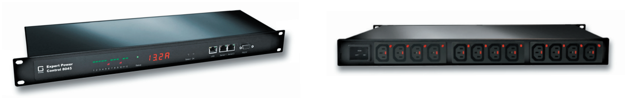
Expert Power Control 8045-2: 12 IEC-Lock outlets on the rear panel prevent unintentional disconnection of the cables
